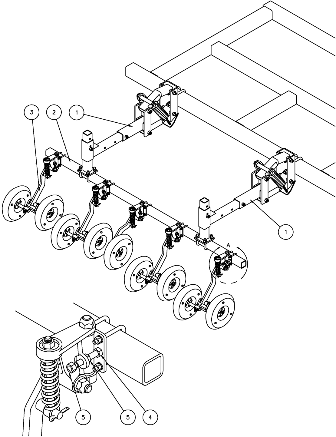
VIEW A
